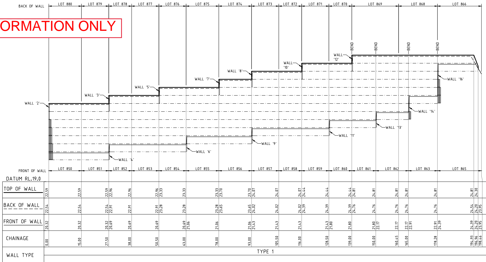
RETAINING WALL '1' HORIZ.-1500 VERT.-150
