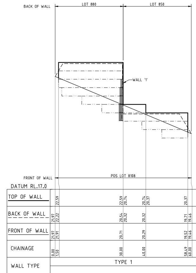
RETAINING WALL '2' HORIZ.-1500 VERT.-150
