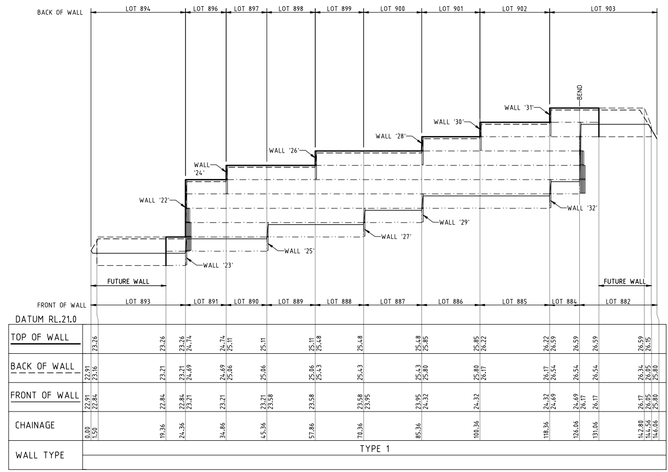
RETAINING WALL '18' HORIZ.-1500 VERT.-150
