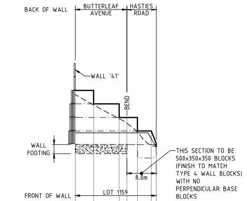
RETAINING WALL '23' HORIZ.-1:500 VERT.-1:50
