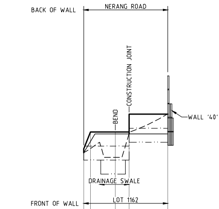
RETAINING WALL '22' HORIZ.-1:500 VERT.-1:50
