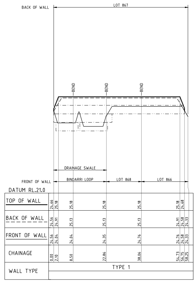
RETAINING WALL '15' HORIZ.-1500 VERT.-150
