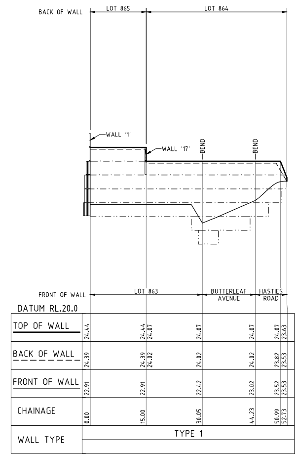
RETAINING WALL '16' HORIZ.-1500 VERT.-150
